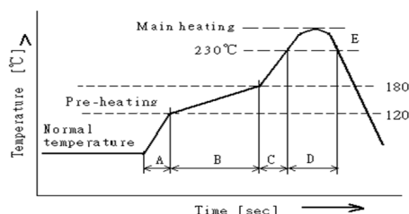
Temperature Profile
